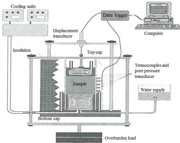
Figure 5 Sketch of LTU freezing-thawing apparatus(Kujala 1991)
