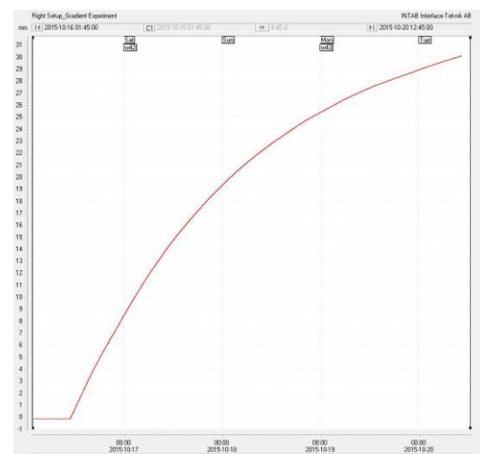
Figure 11 Frost heave (mm) LVDT readings
